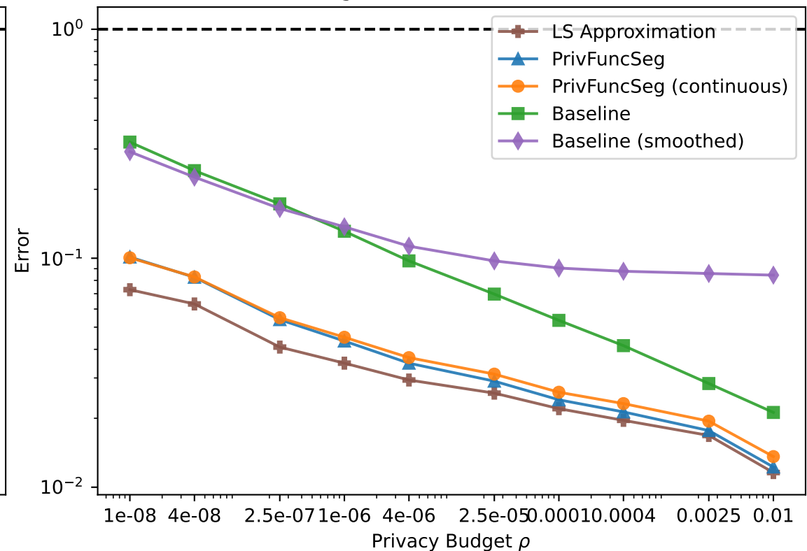
Degree-4 Monomial Basis
